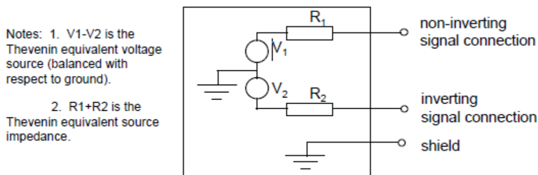
FIGURE 16a. Equivalent circuit of ASI or MSI when sending a LB signal
