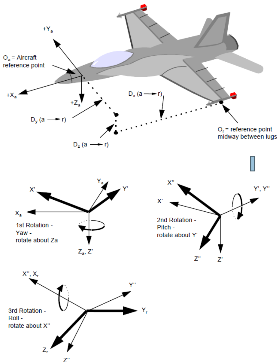
FIGURE B-6. Aircraft-store alignment
