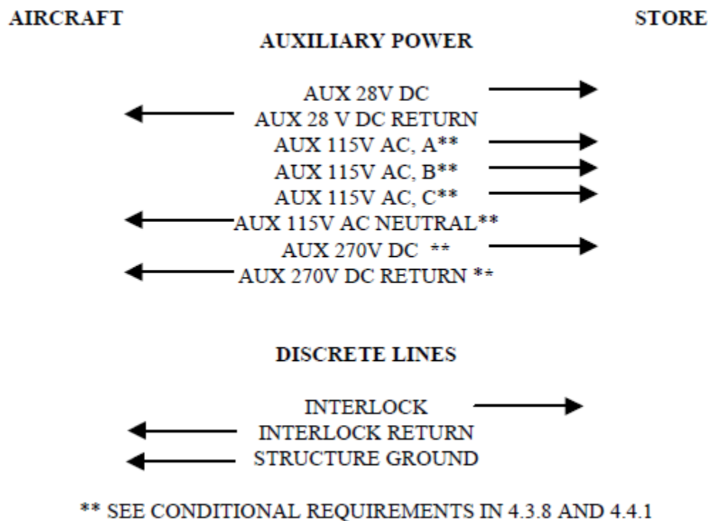
FIGURE 3. Auxiliary Power Signal Set
