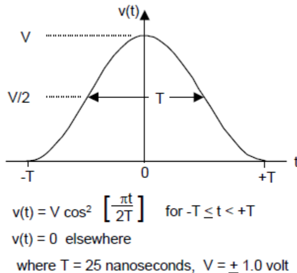
FIGURE 5a. Cosine-squared T signal
