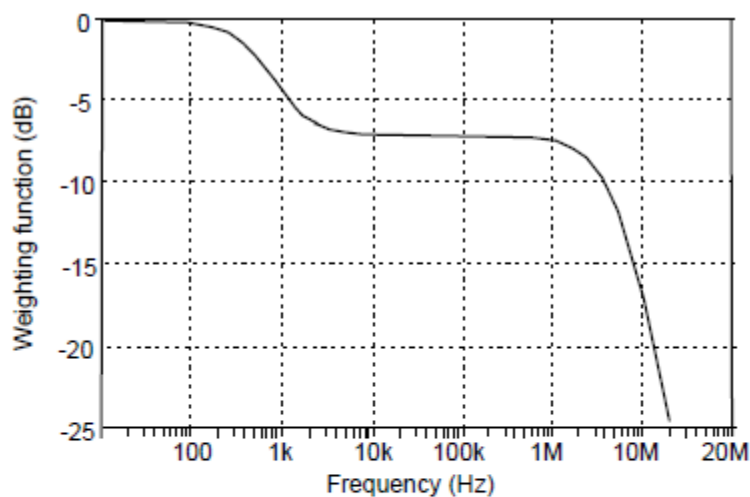
FIGURE 10. Random noise weighting function
