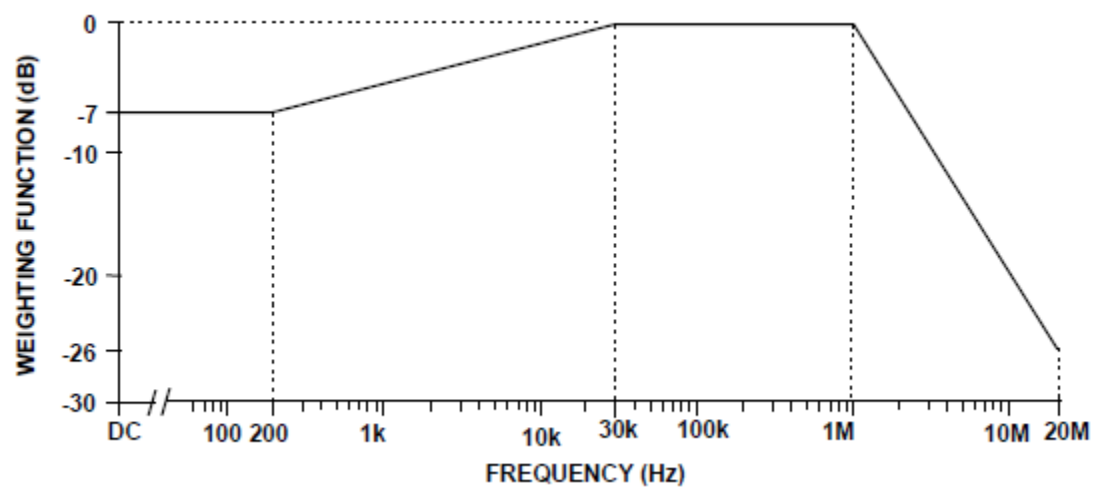
FIGURE 12. Common mode noise weighting function
