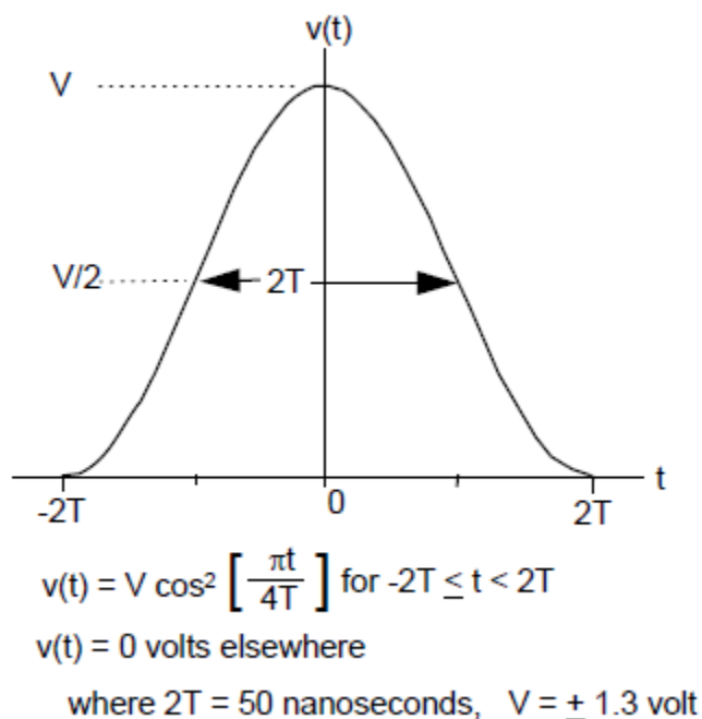
FIGURE 6a. Cosine-squared 2T signal
