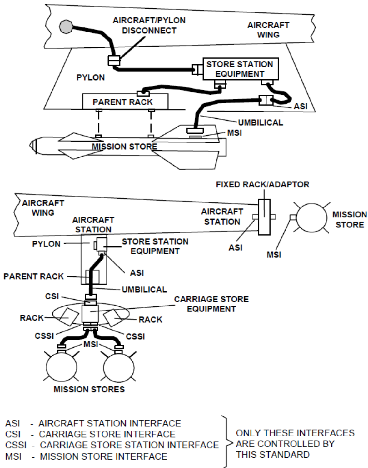
FIGURE 1. Aircraft-Store Configuration Examples
