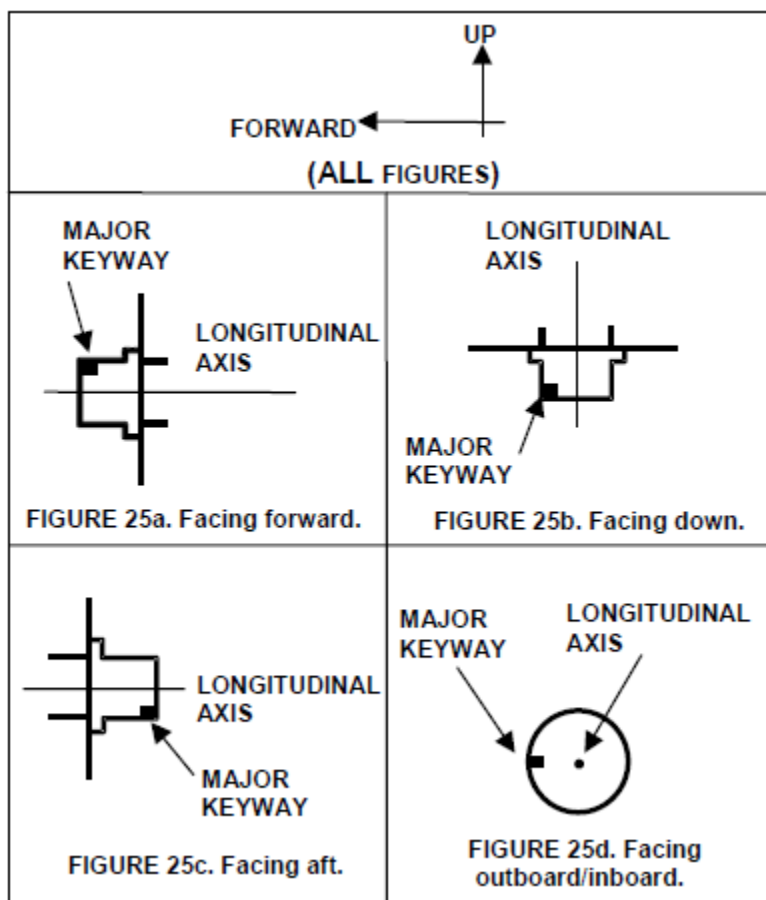
FIGURE 25. Connector orientation
