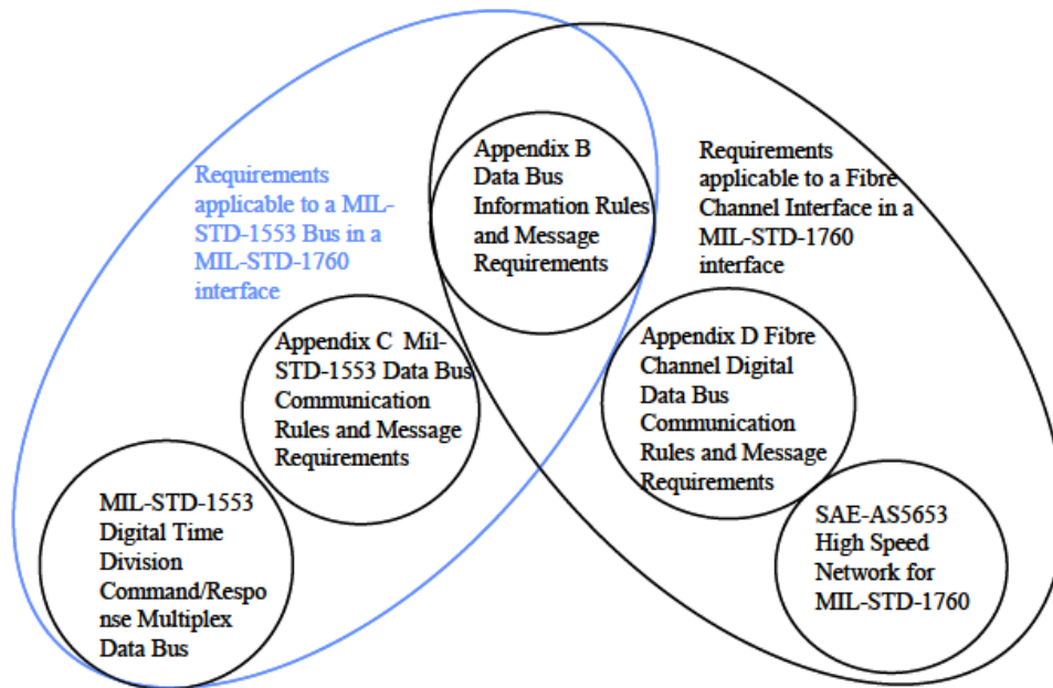
FIGURE B-1. Relationship between Appendix B, C and D
