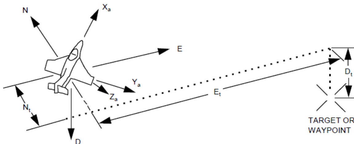
FIGURE B-7. Store body axis system
