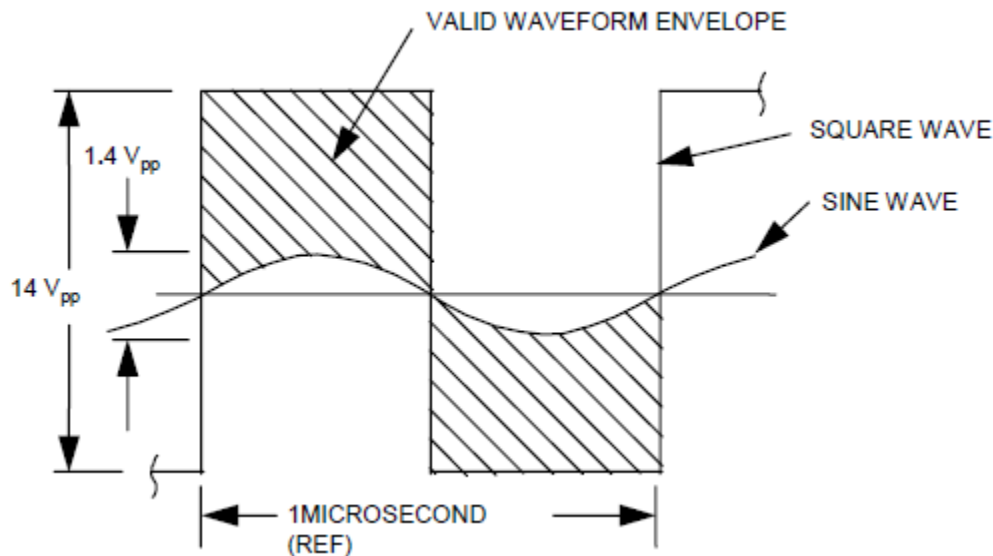
FIGURE 14. ASI output waveform envelope
