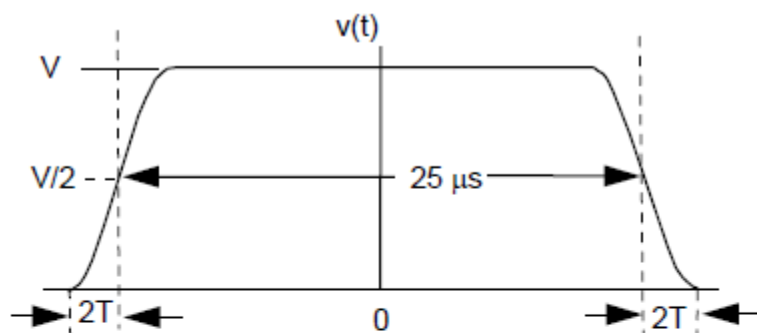
FIGURE 7. 2T Bar signal requirements (1.0 V)
