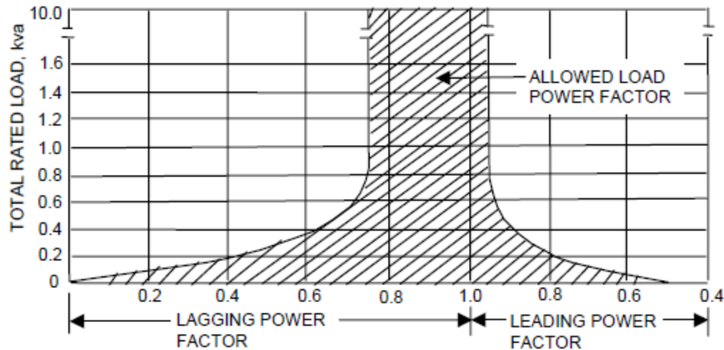
FIGURE 20. Power factor limits
