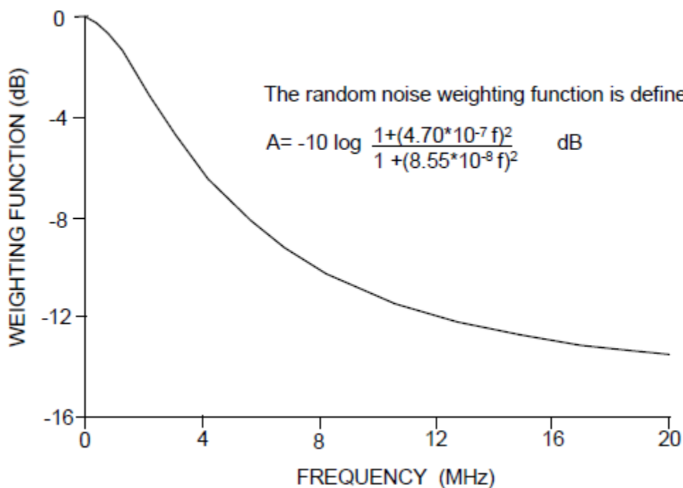
FIGURE 10. Random noise weighting function
