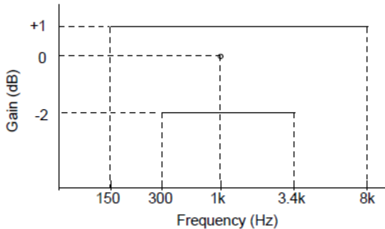
FIGURE 15. Gain misequalization envelope (aircraft, LB)
