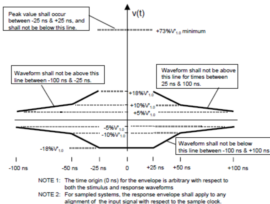
FIGURE 5b. Allowed response envelope for cosine-squared T signal
