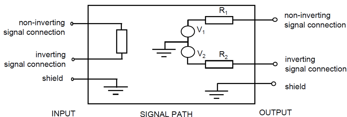
FIGURE 23a. Equivalent circuit for LB passive signal path
