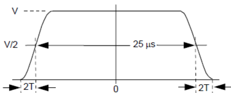
FIGURE 6. Cosine-squared 2T signal requirements
