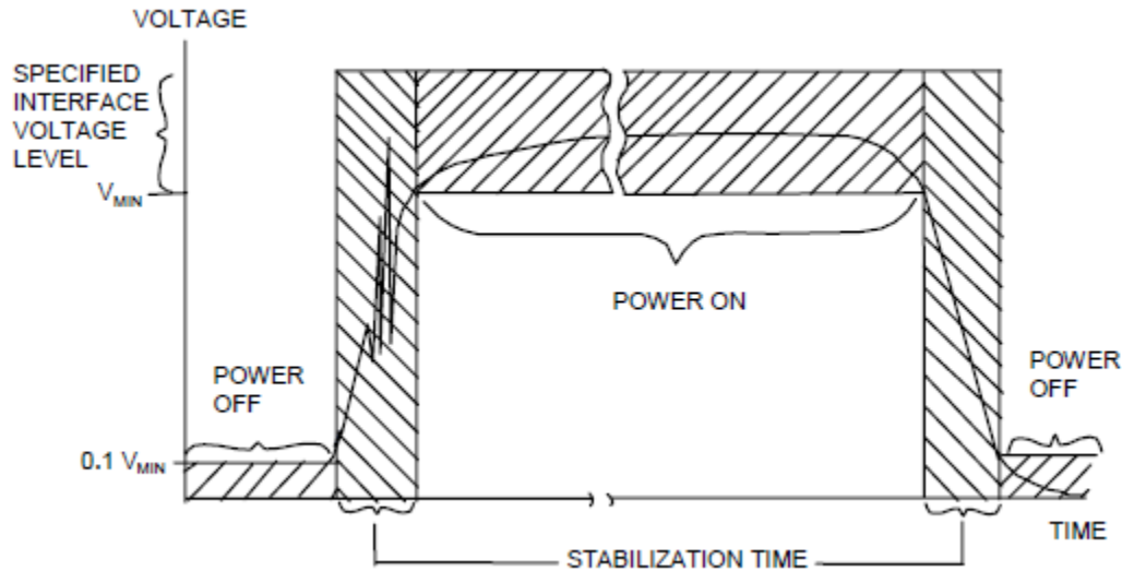
FIGURE 19. Stabilization time
