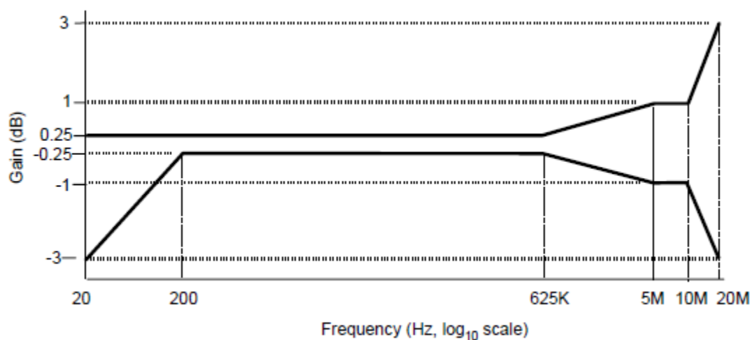
FIGURE 8. 2T Bar signal requirements (1.3V)
