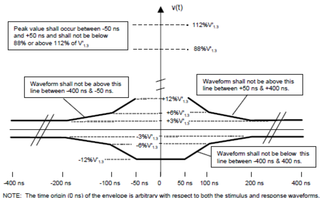
FIGURE 6b. Allowed response envelope for cosine-squared 2T signal
