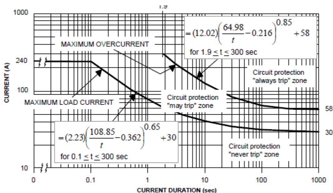
FIGURE 18a. Auxiliary interface current level for 28 V dc and 115 V ac power
