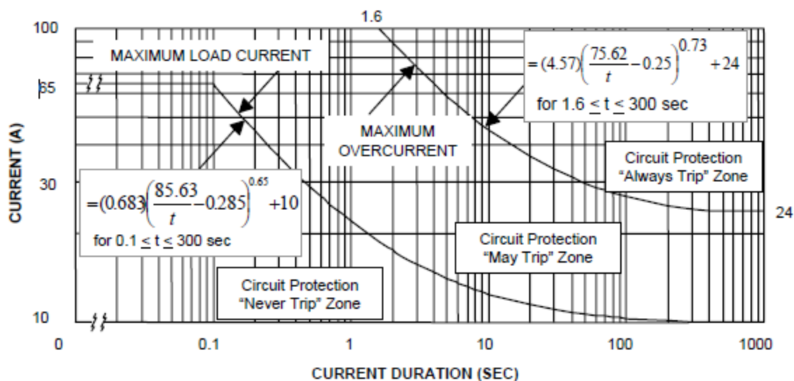
FIGURE 17a. Primary interface current level for 28 V dc and 115 V ac power
