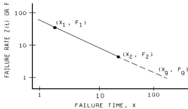
FIGURE 2. Failure rate versus time.
