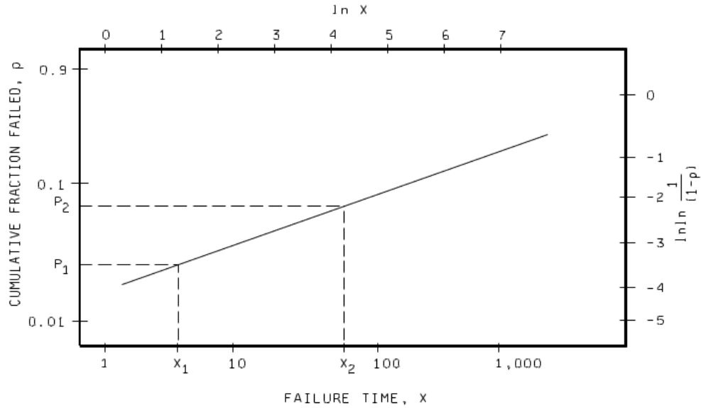
FIGURE 1. Typical Weibull plot.
