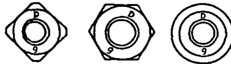
METRIC SQUARE, HEX, AND ROUND WELD NUTS (DEPRESSED LETTER "D" AND CLASS NO.)
