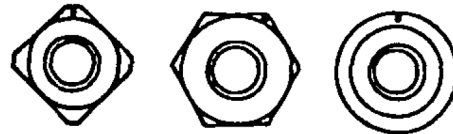
AMERICAN STANDARD SQUARE, HEX, AND ROUND WELD NUT (SMALL RAISED DOR ON CHAMFER)
