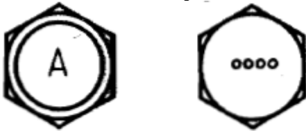
Head markings
