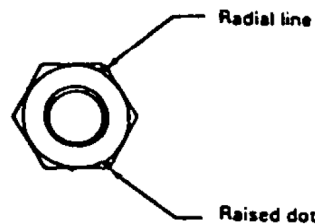
GRADE 5 NEX NUTS (ONE RAISED RADIAL LIVE 120° COUNTERCLOCKWISE FROM ONE RAISED DOT ON CHAMFER)
