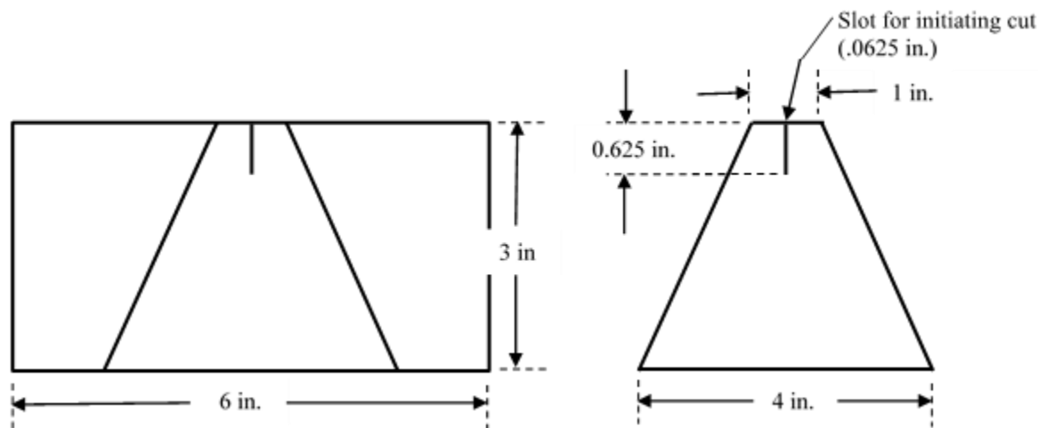
FIGURE 2. Diagram of marked trapezoid specimen.
