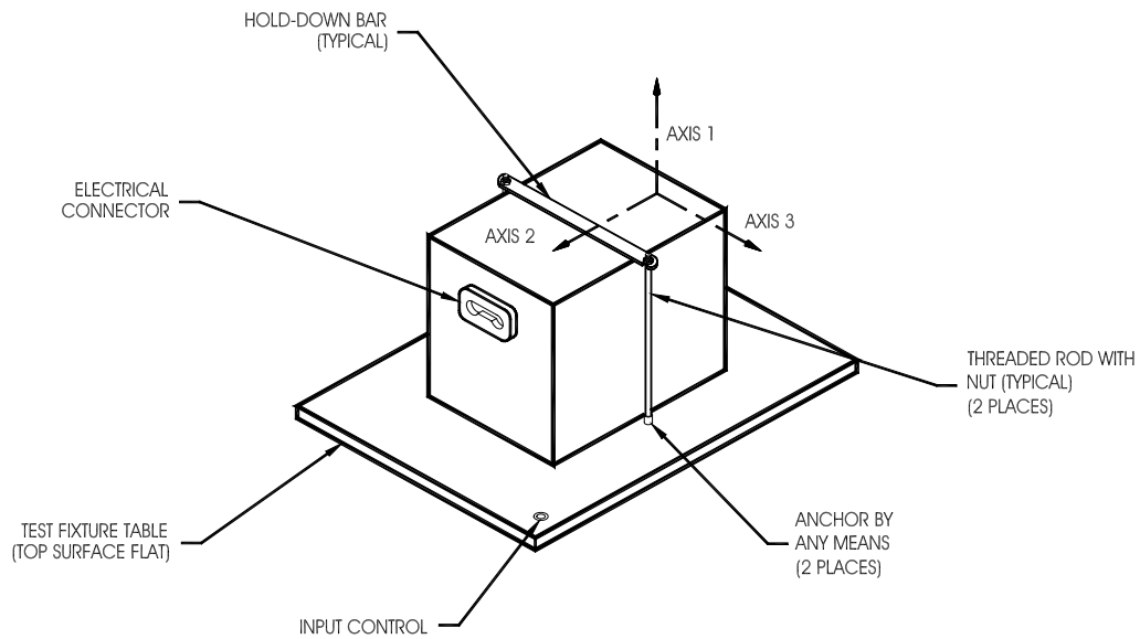
CONVENTIONAL MOUNTED BATTERY
