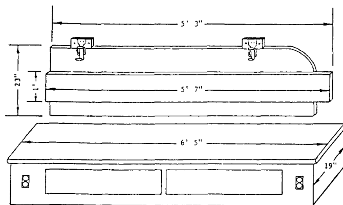
APPENDIX FIGURE 1 COMBINATION BACKREST/LITTER SUPPORT PANEL - PLAN AA
