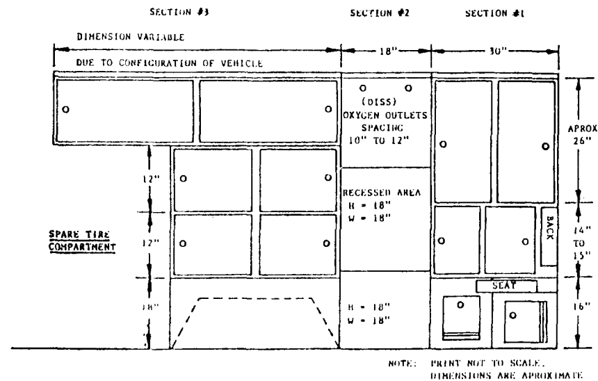
APPENDIX FIGURE 3 STREETSIDE CABINETRY - PLAN AN
