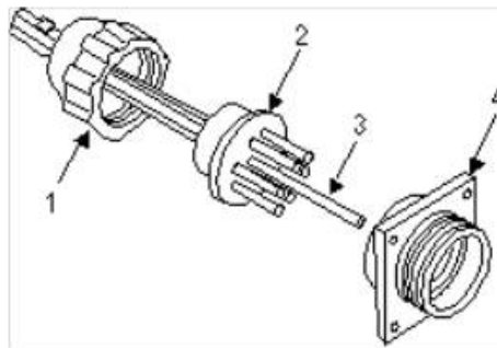
Figure 1. 24-volt Connector Receptacle
