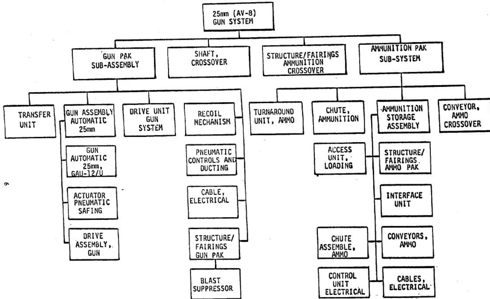
FIGURE 1. Breakdown structure.
