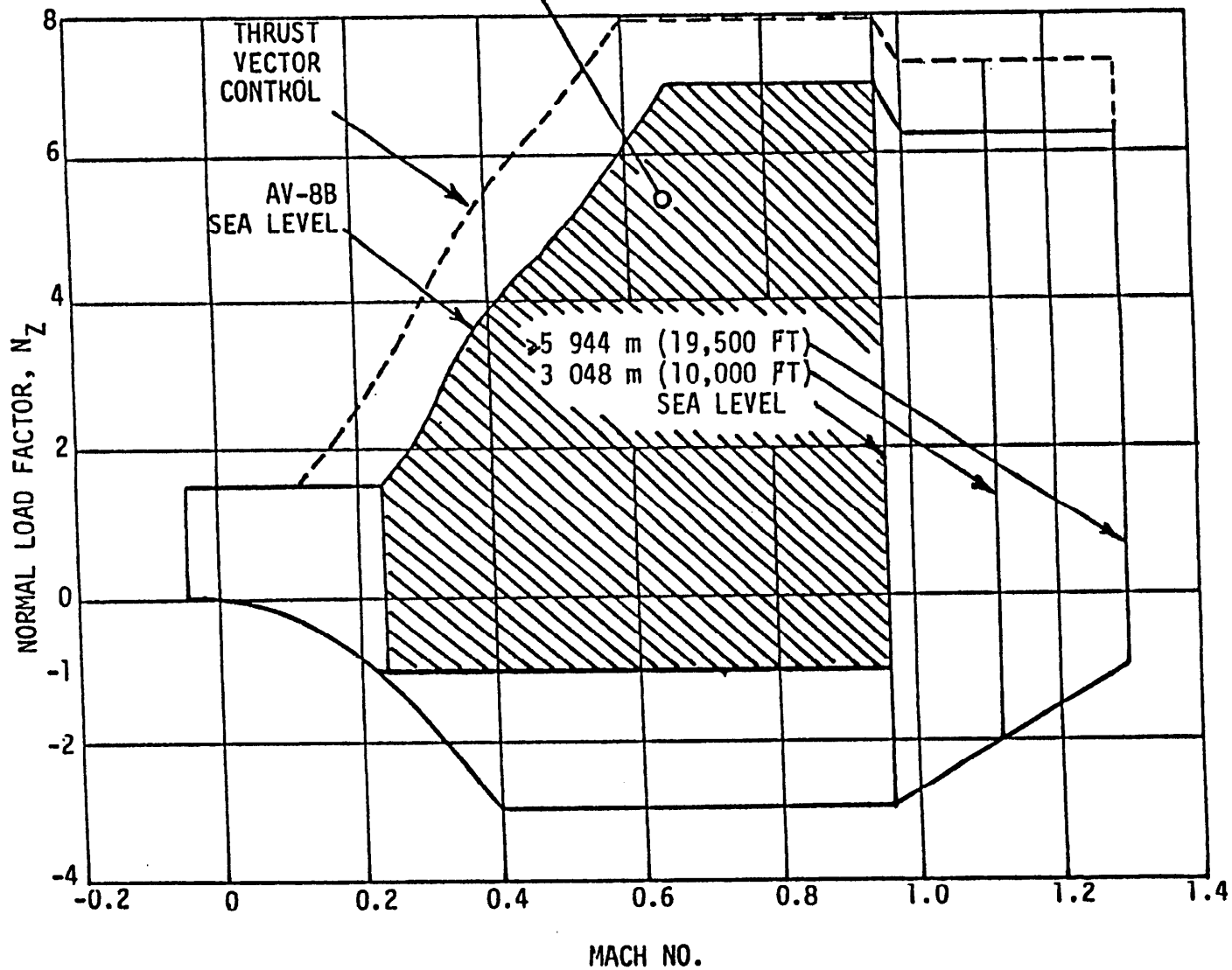
FIGURE 3. AV-8B flight strength envelope.
