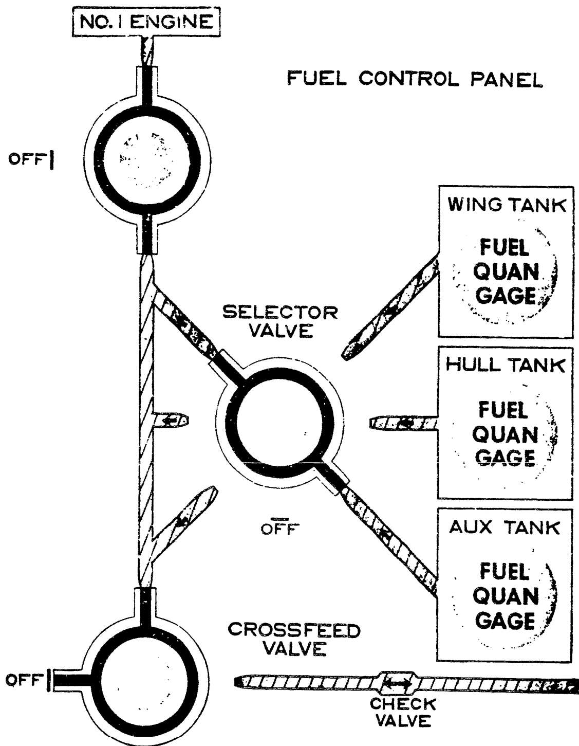
FIGURE 3. Fuel control panel
