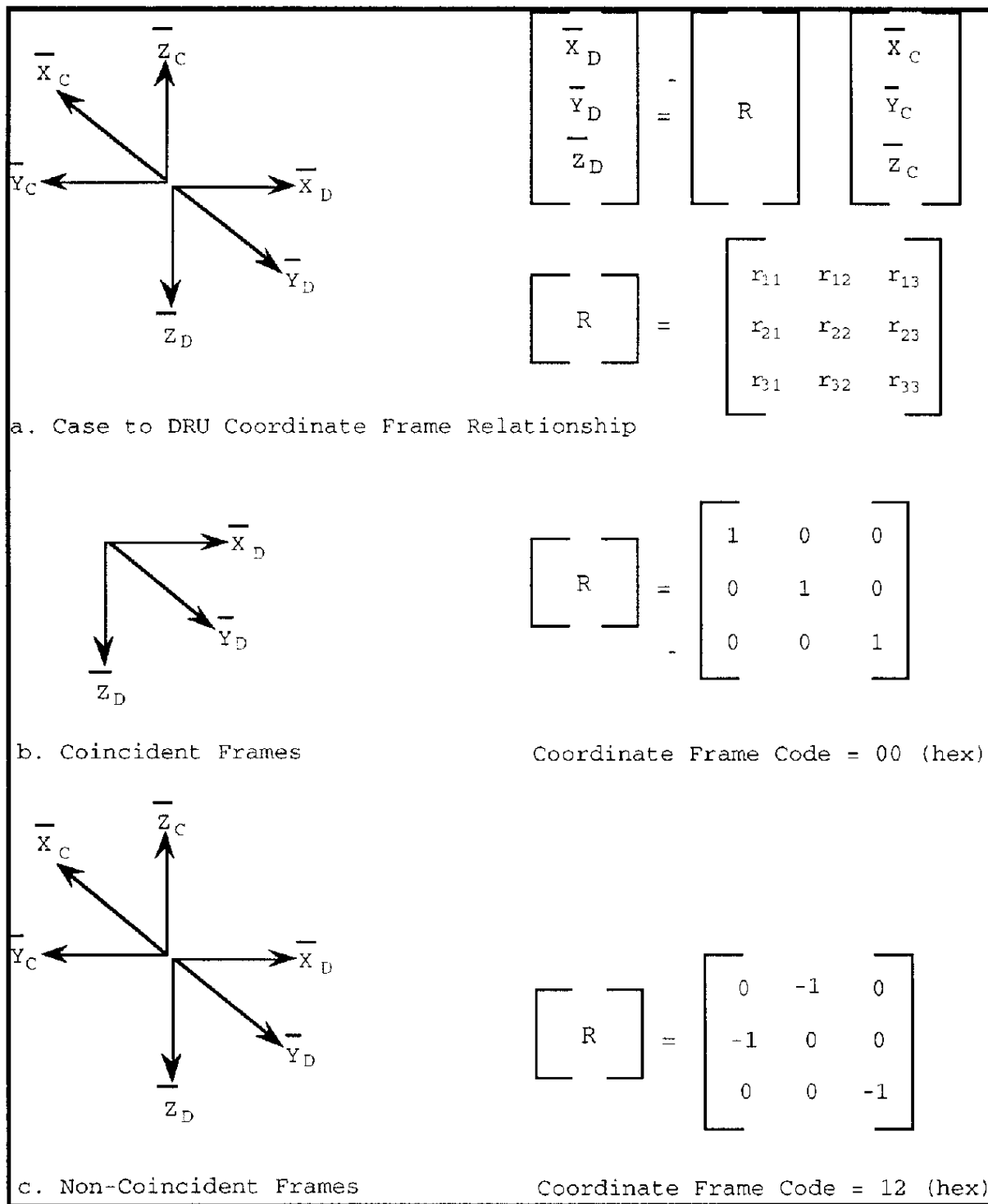
Figure 8. DRUH coordinate frame.
