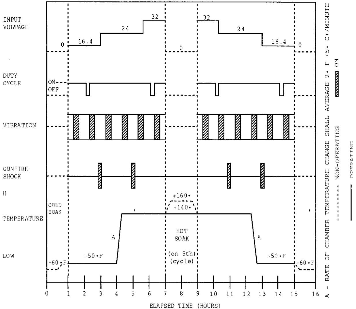
Figure 4. Chamber test cycle.
