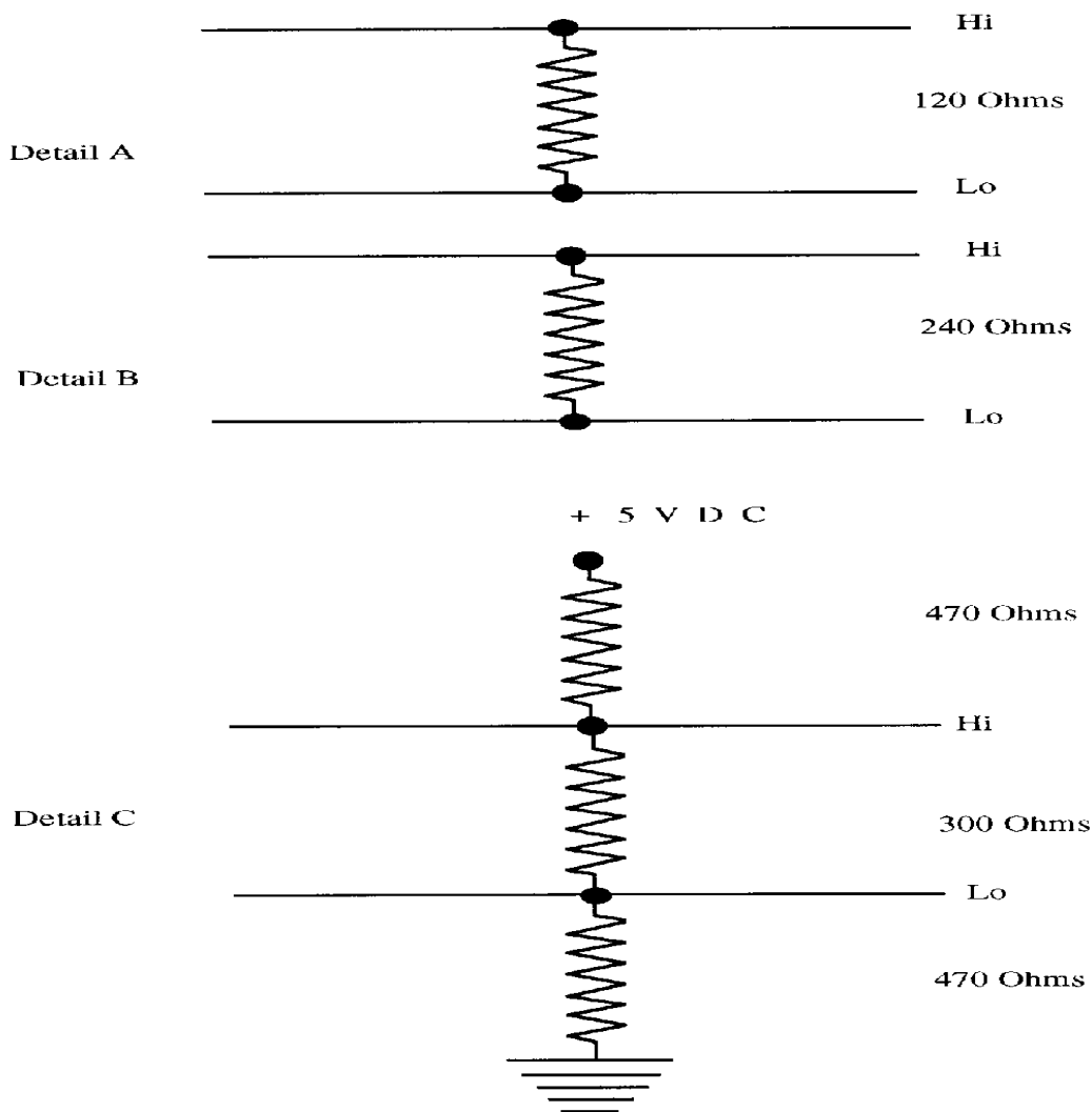
Figure 1. Termination details.
