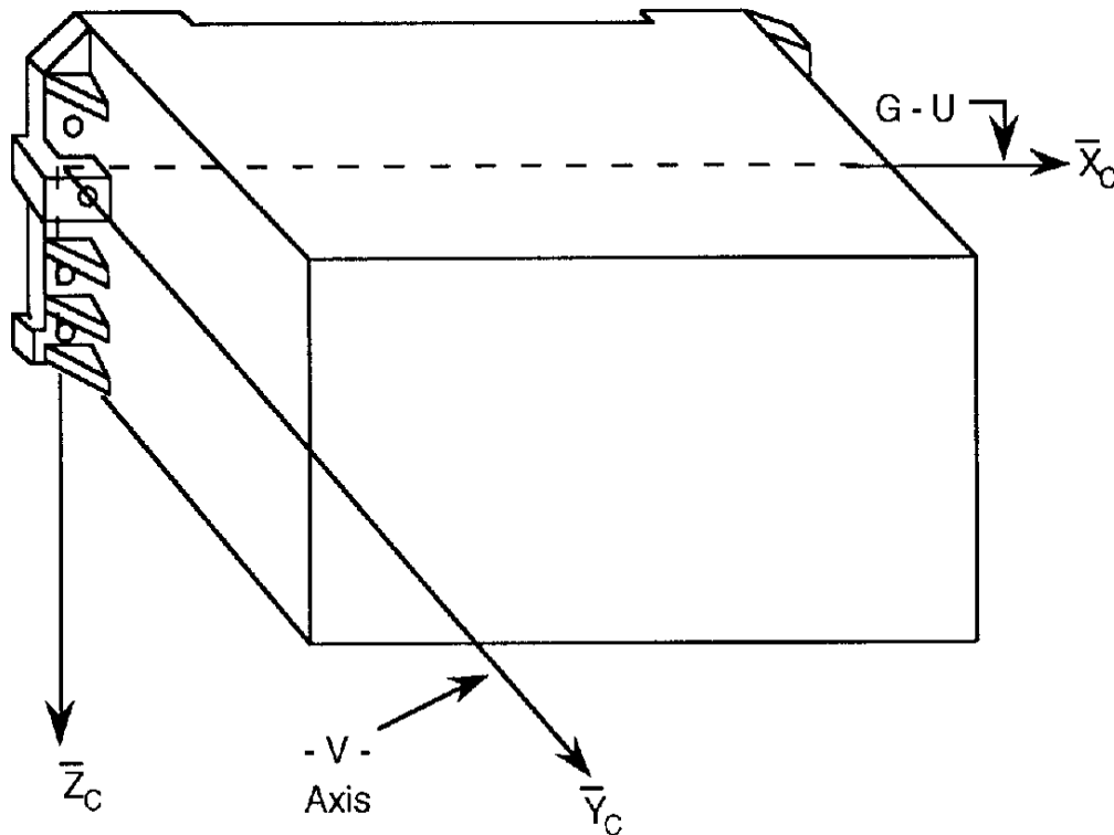
Figure 7. DRUH case coordinate frame.
