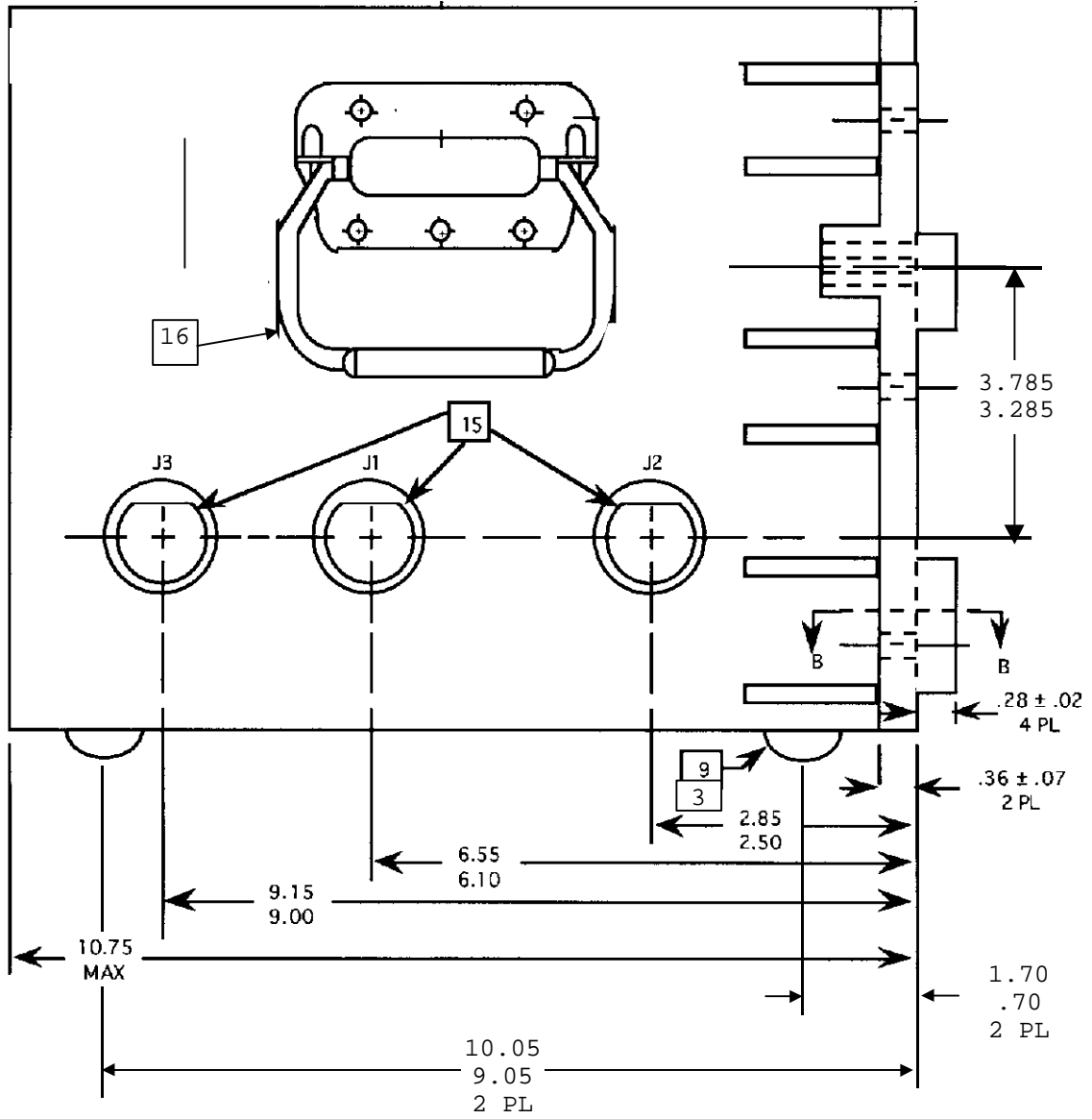
FIGURE F-1. DRUH right side.
