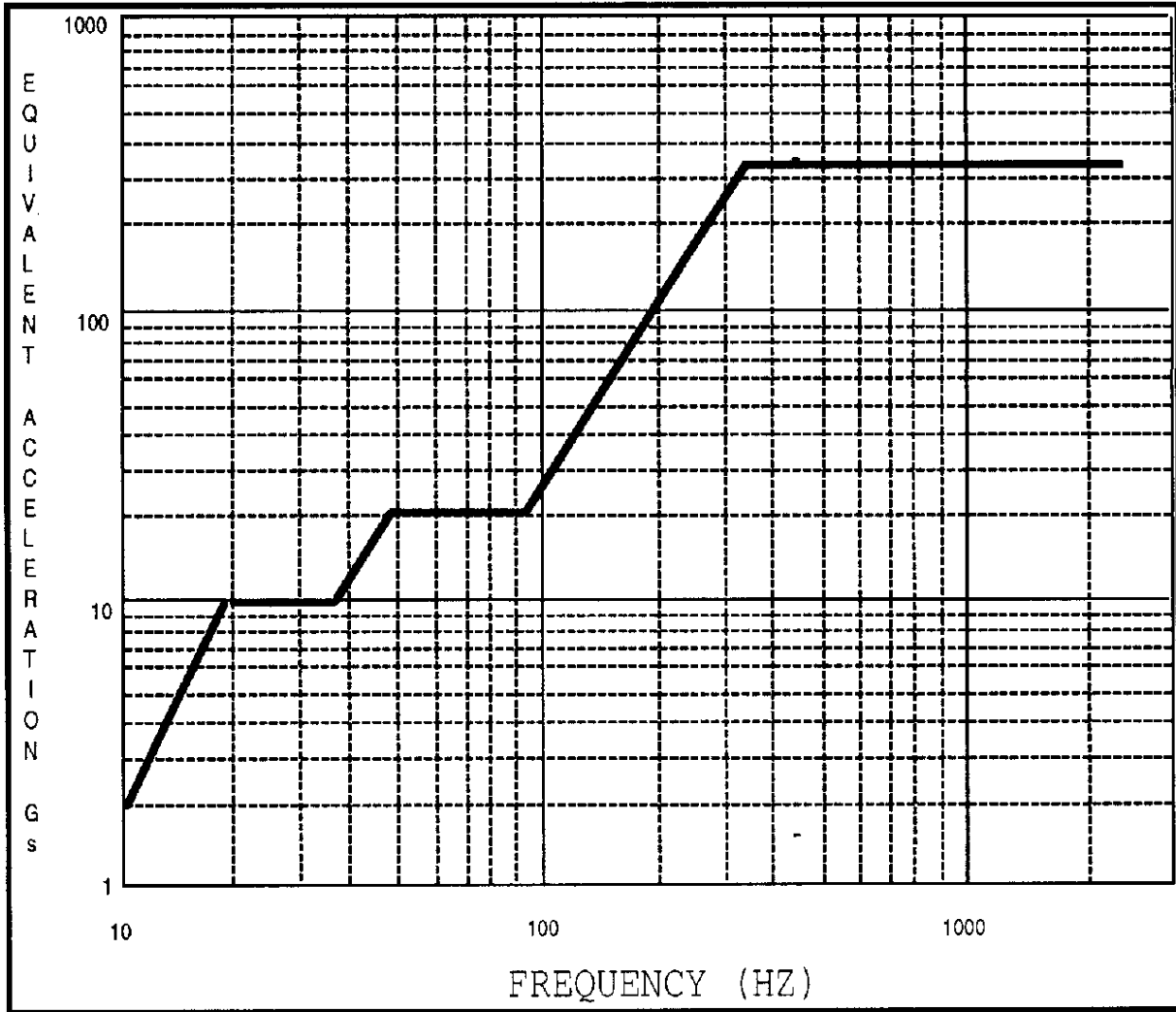
Spectrum Break Points
