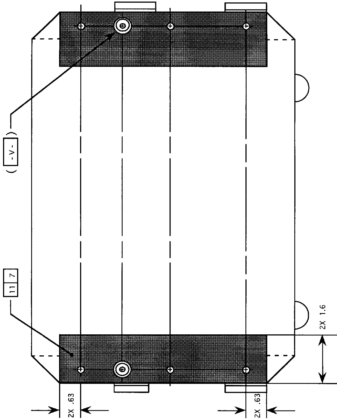
FIGURE F-3. DRUH back/mounting surface.
