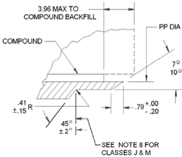
DETAIL C ENLARGED
